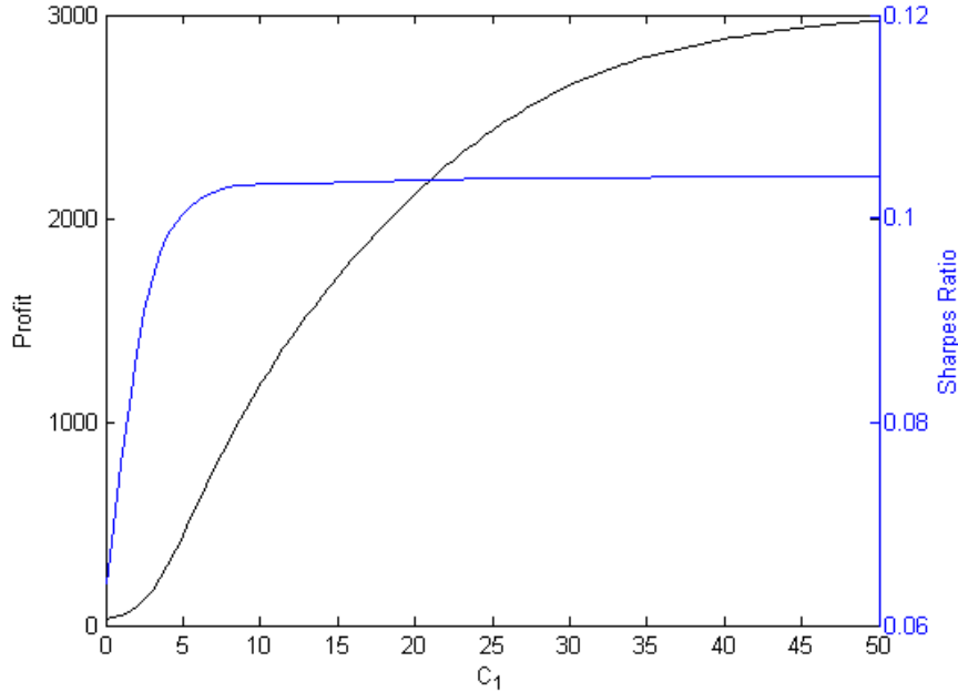
Figure 4.4: Effect of c_1 on profit and Sharpe's Ratio - The higher values of the parameter c_1 give more weight to assets that have been loosing several times in a row
